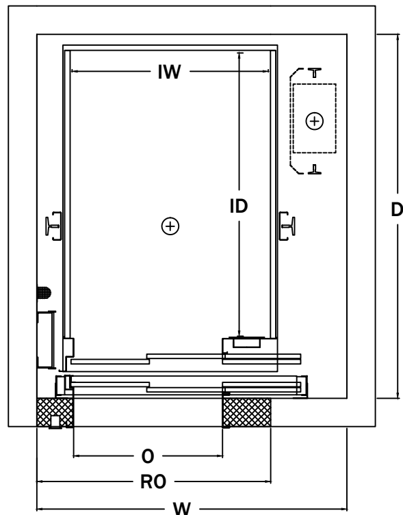
Left Hand Opening Shown Right Hand Opposite
