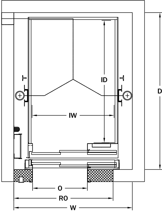
Left Hand Opening Shown Right Hand Opposite
