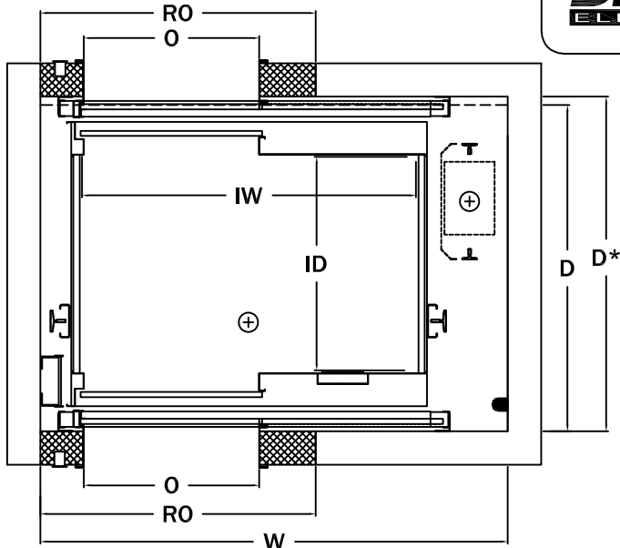
Left Hand Opening Shown Right Hand Opposite
