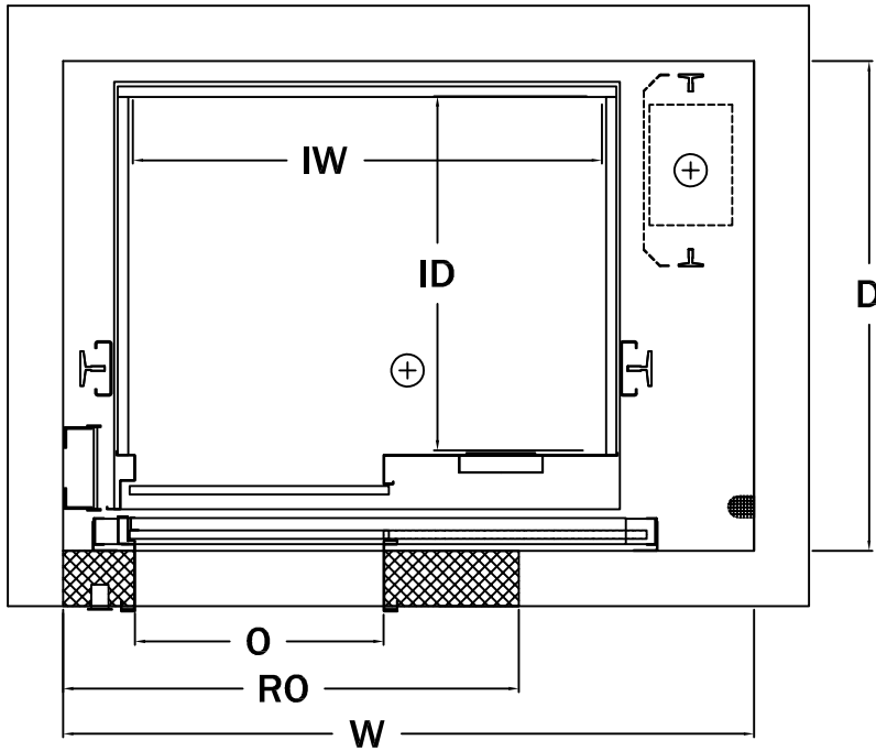
Left Hand Opening Shown Right Hand Opposite
